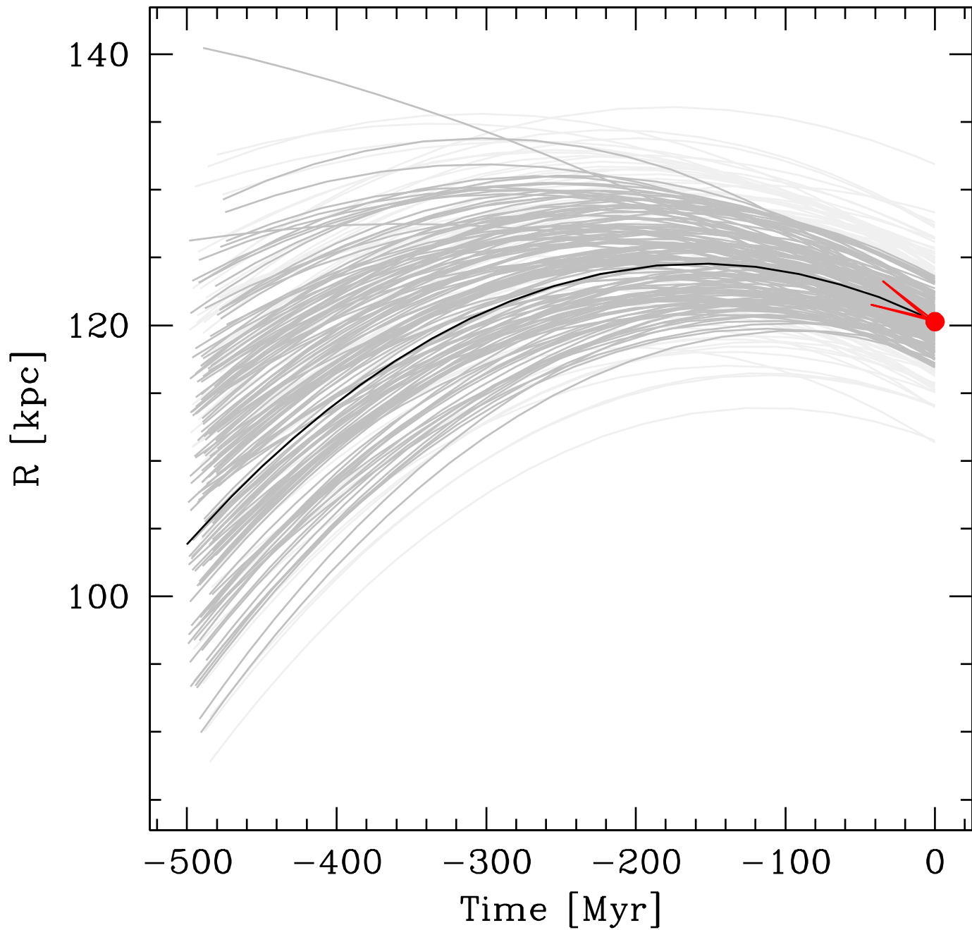
Galactocentric Distance vs. Time
