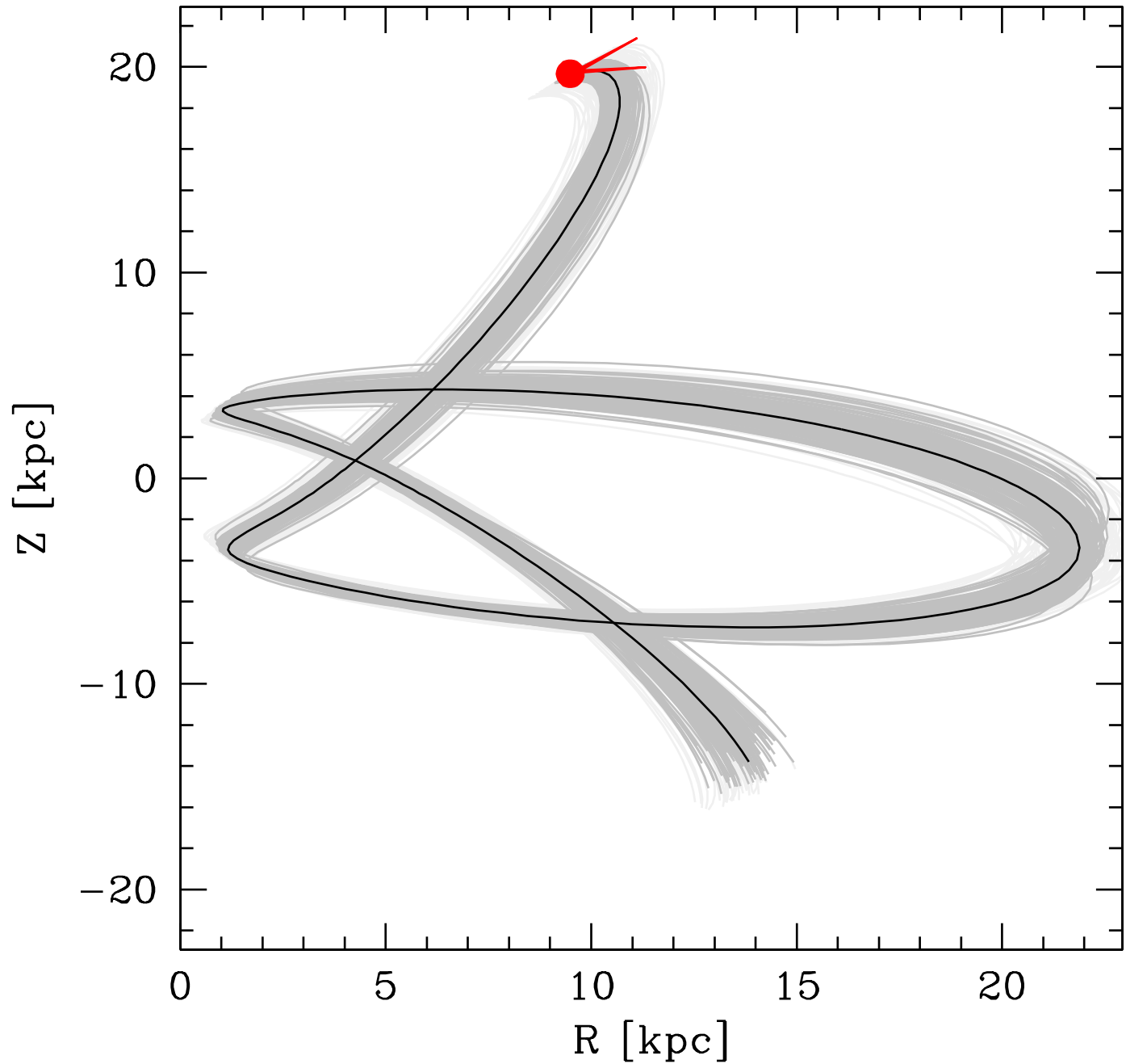
Orbit in Meridional Plane
