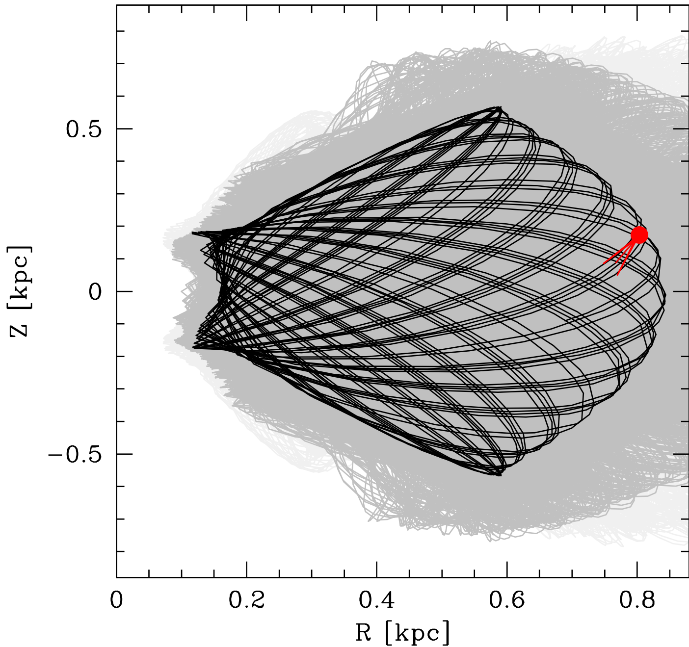
Orbit in Meridional Plane
