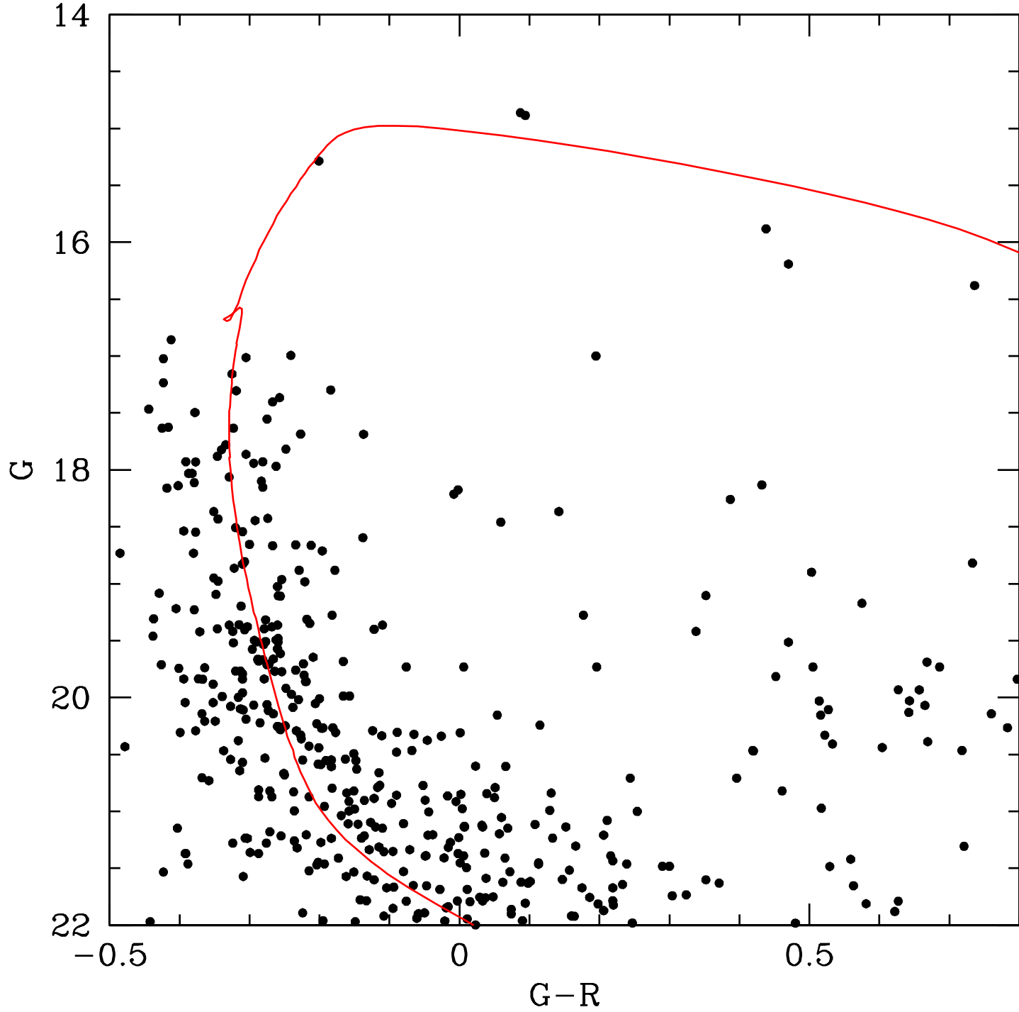
NGC 256
