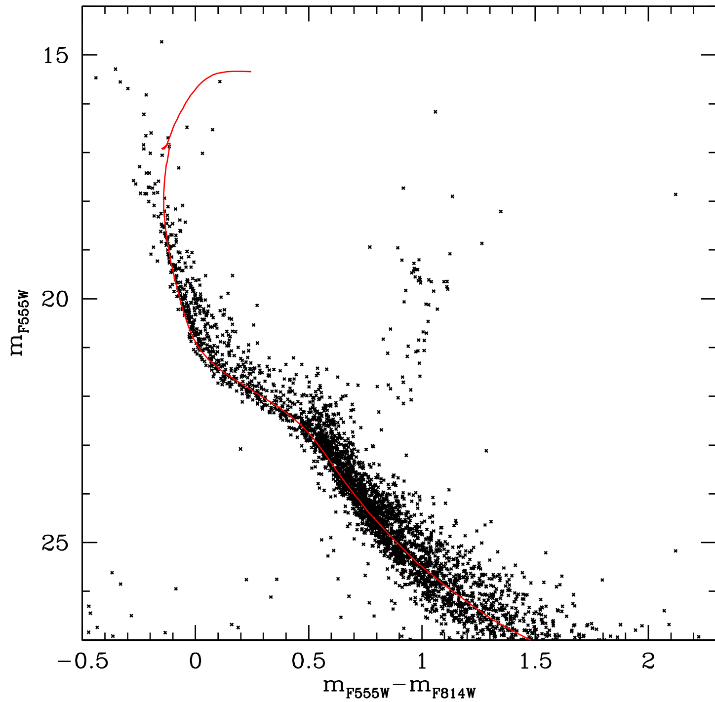
NGC 299
