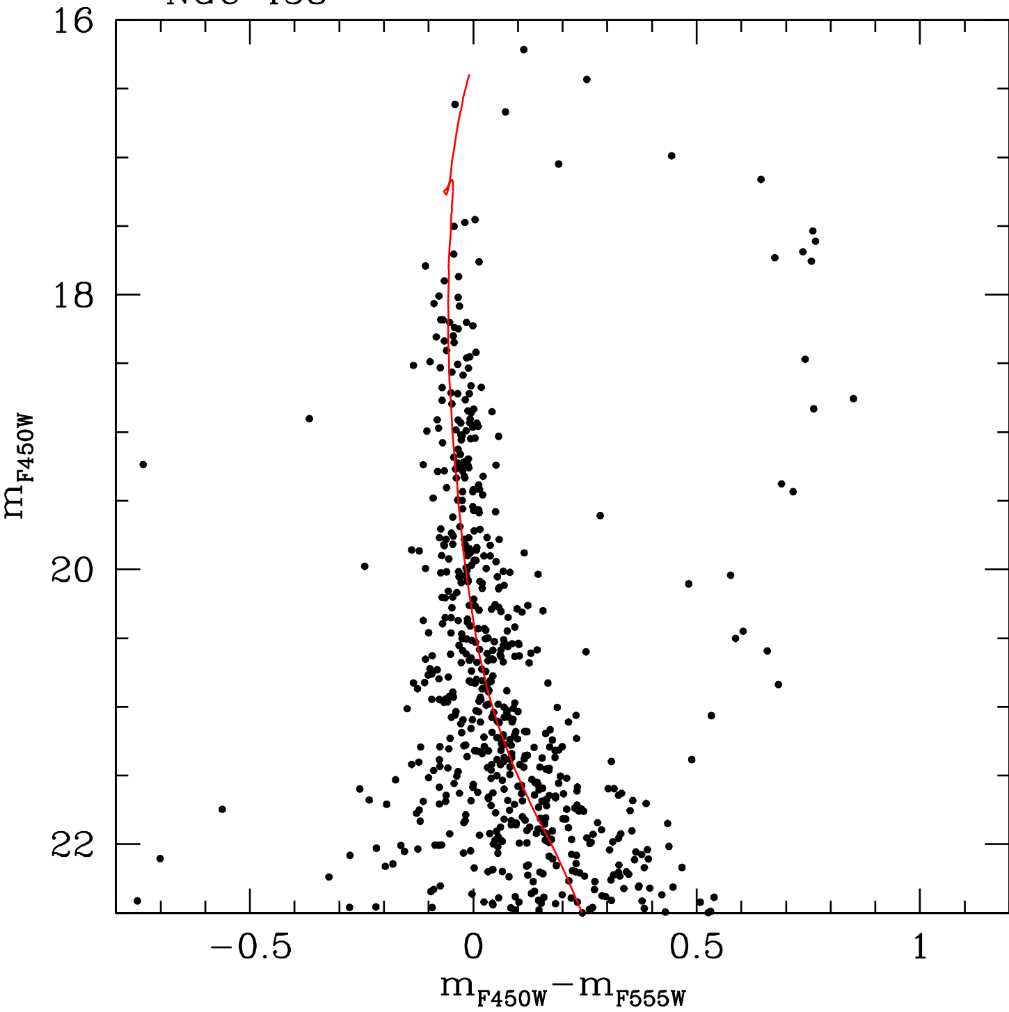
NGC 458
