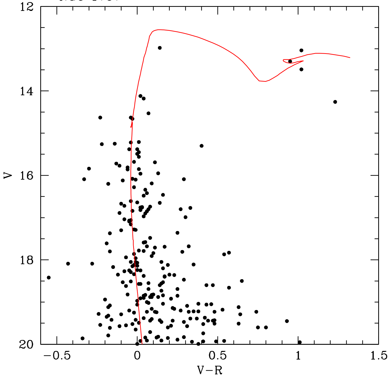
NGC 1767
