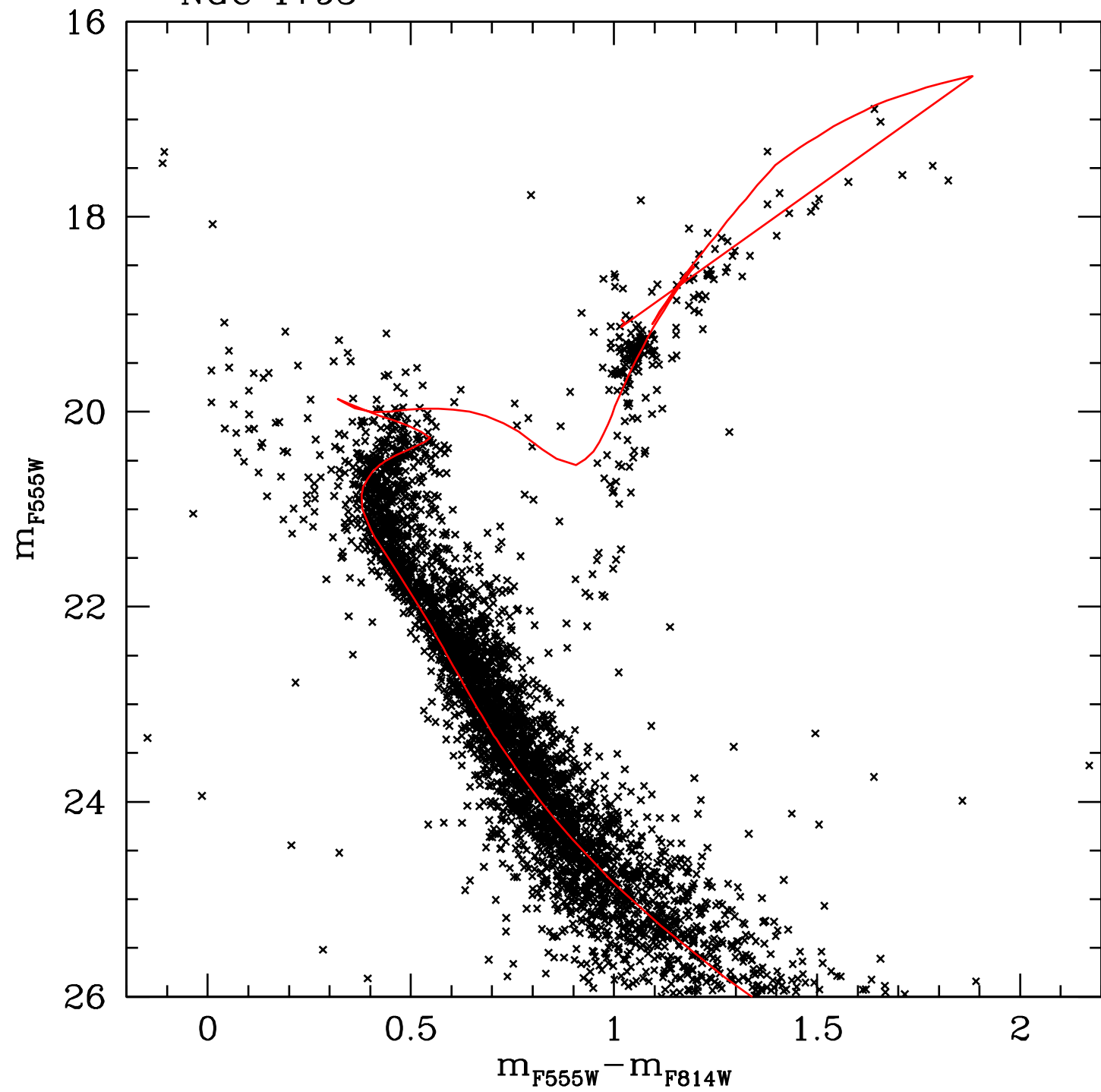
NGC 1795
