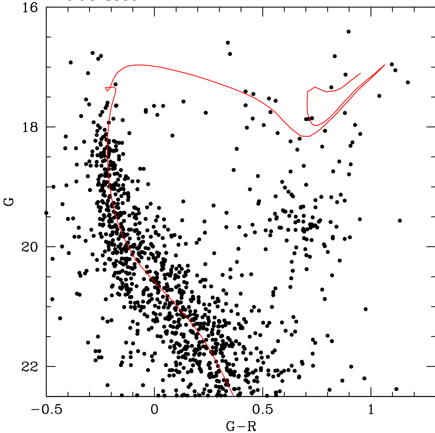
NGC 1830
