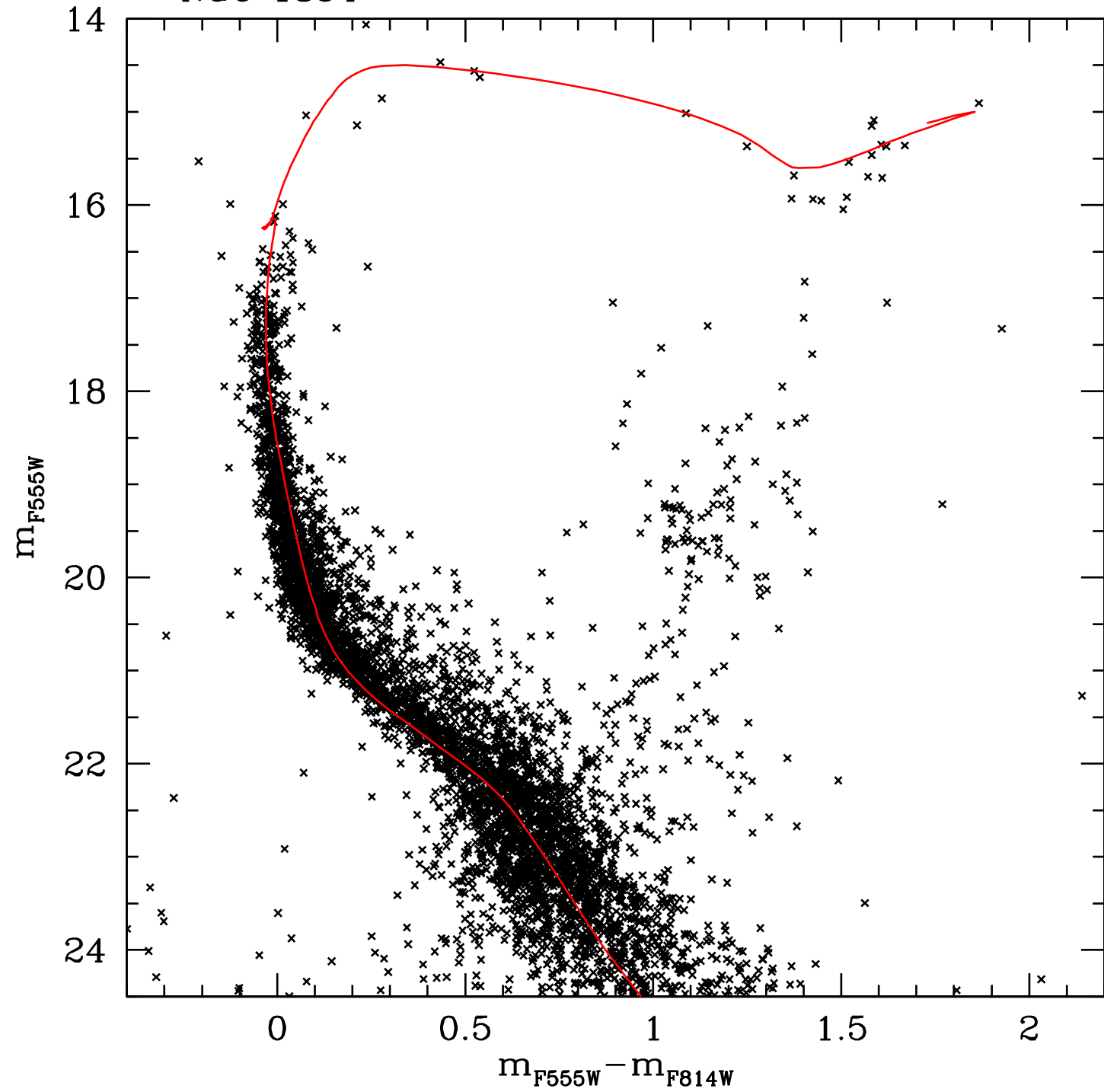
NGC 1854
