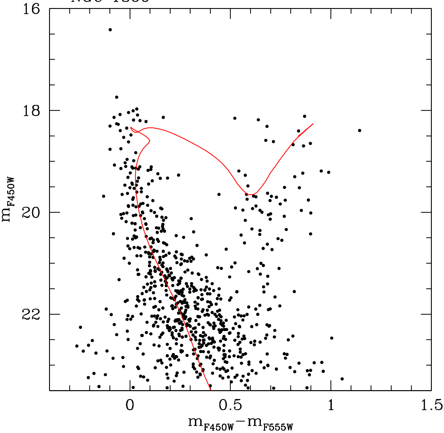
NGC 1860
