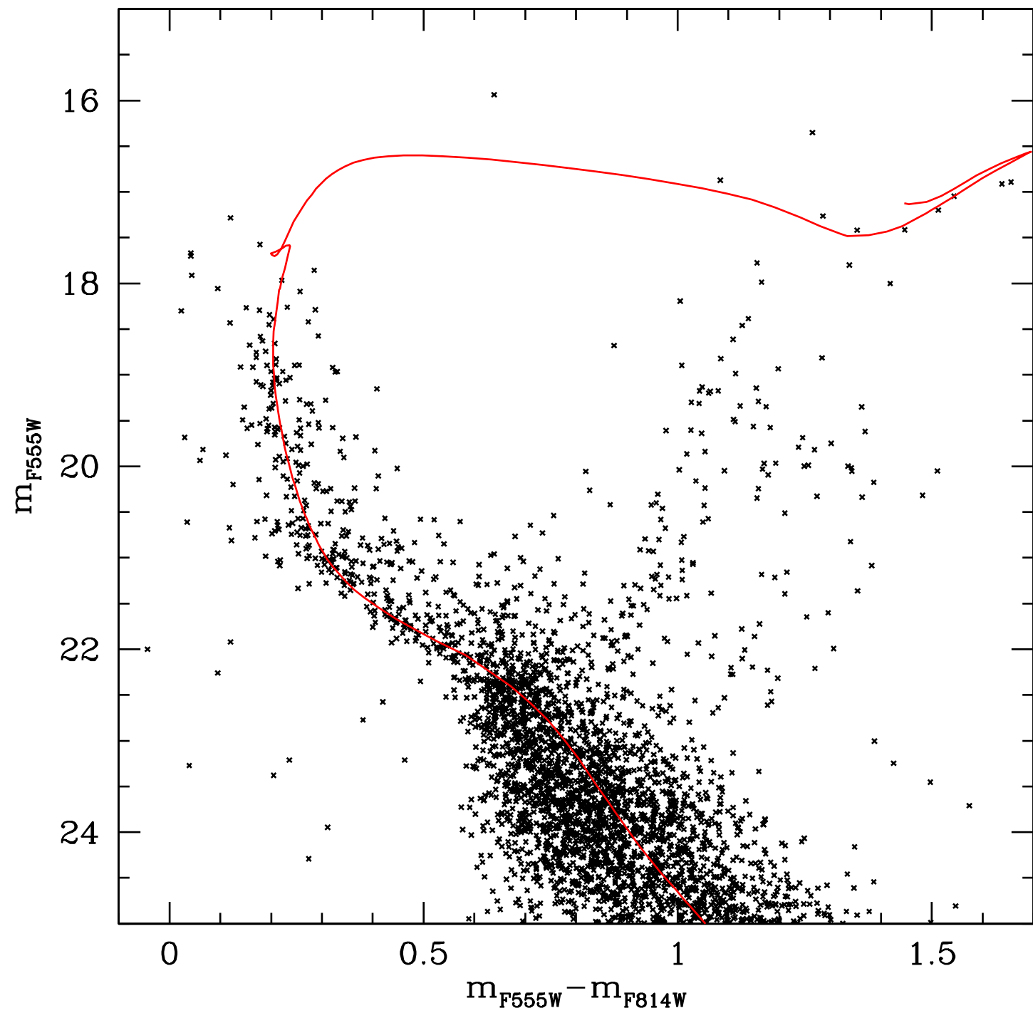
NGC 1938
