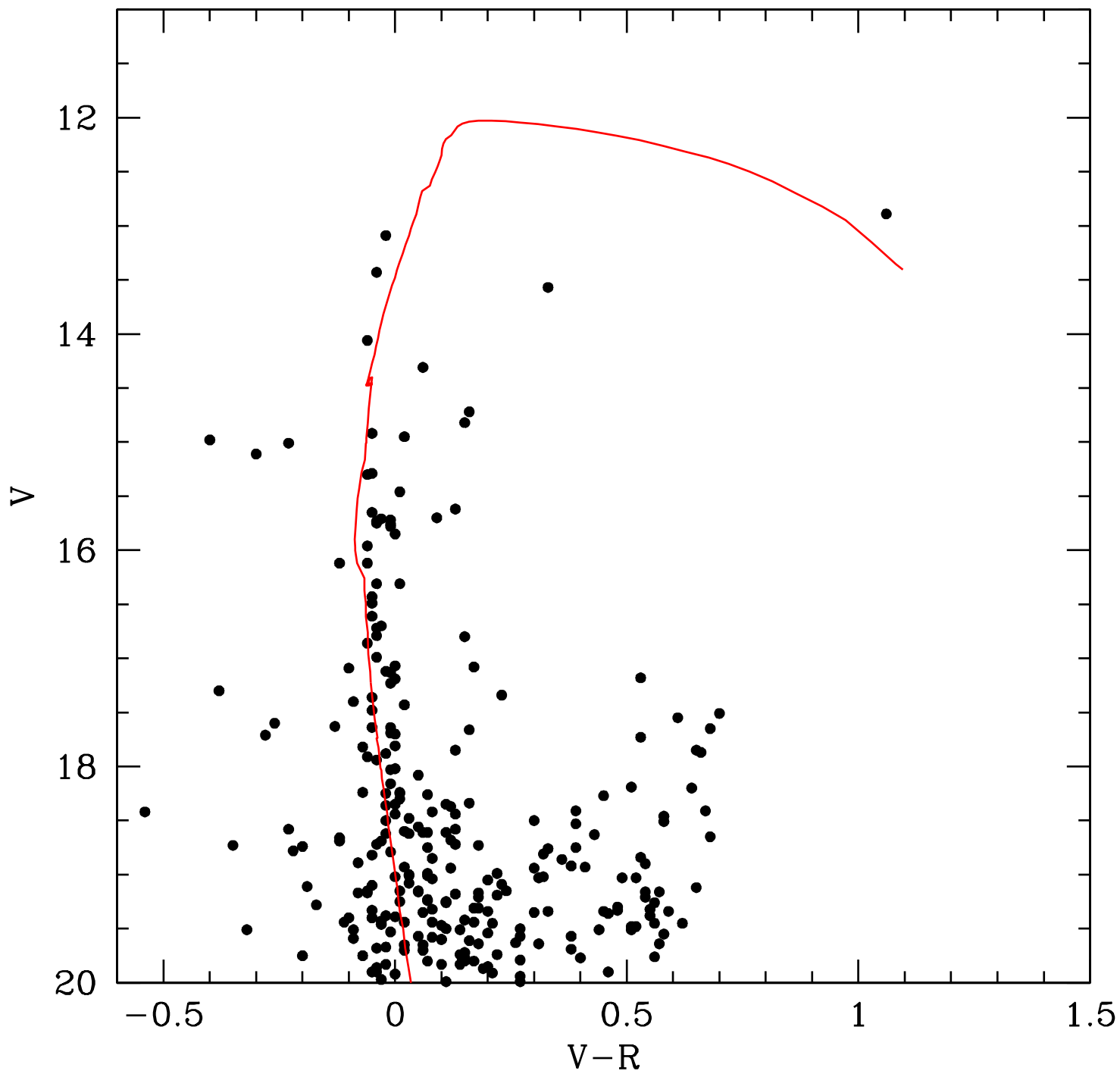
NGC 1994
