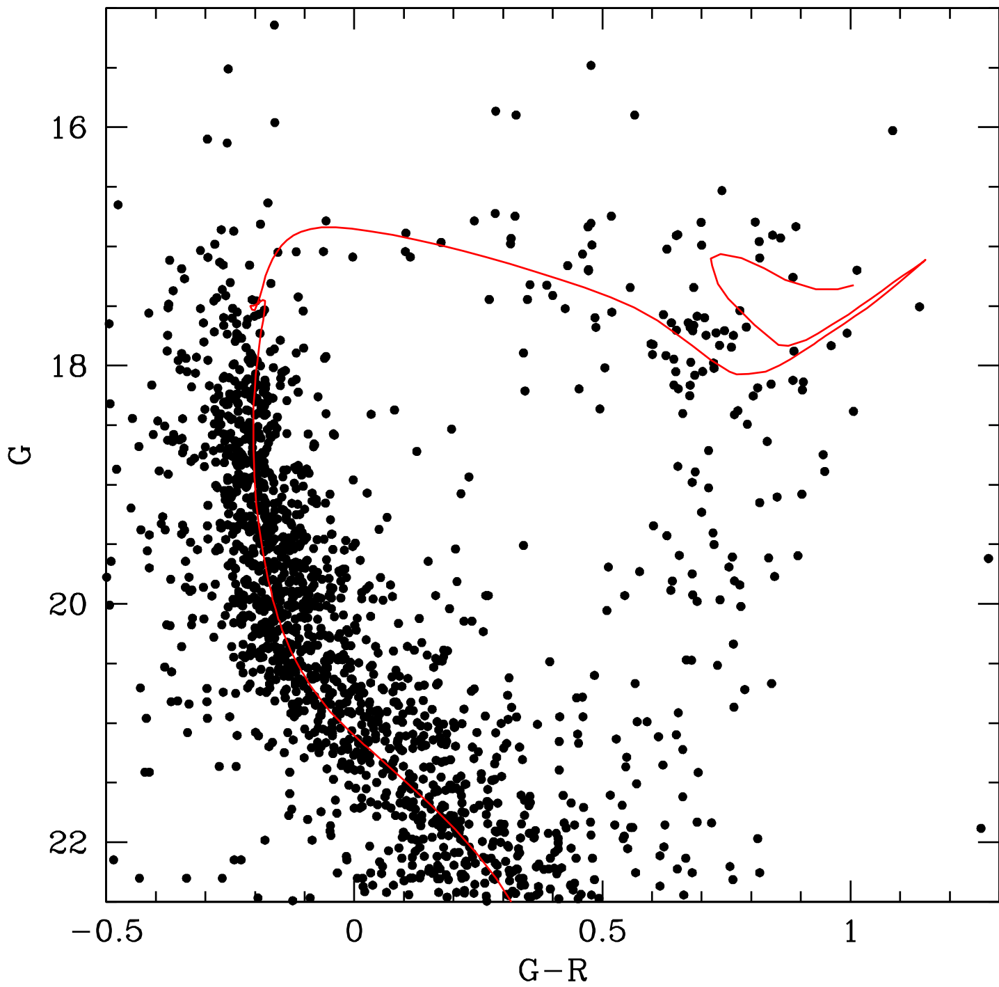
NGC 2134
