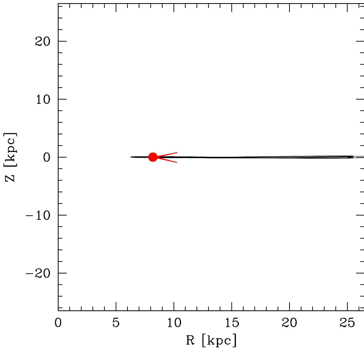
Orbit in Meridional Plane
