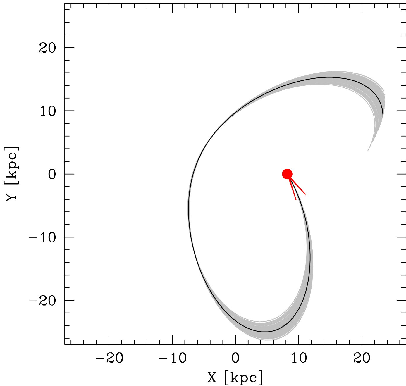
Orbit in Galactic Plane
