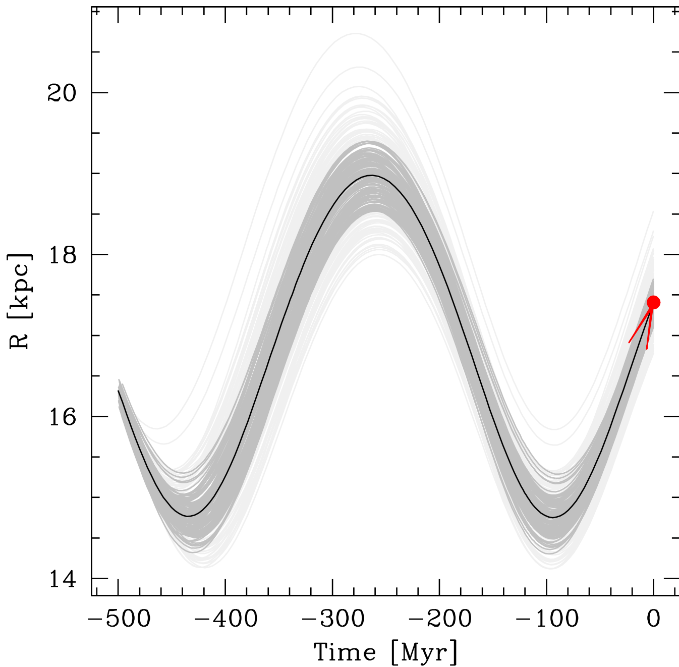
Galactocentric Distance vs. Time
