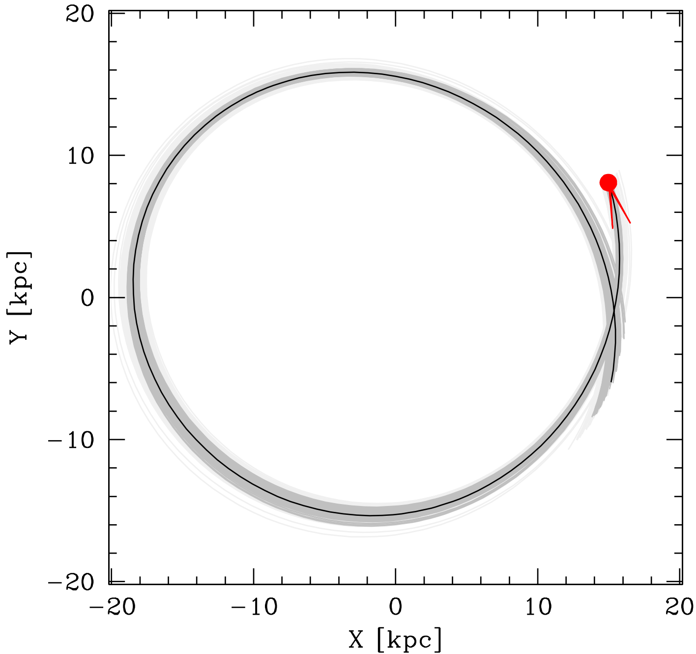
Orbit in Galactic Plane
