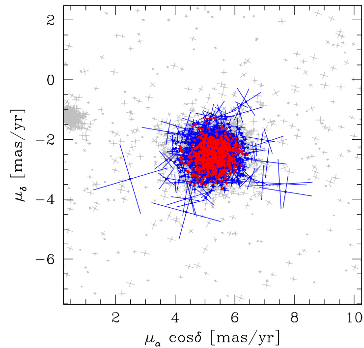
NGC 104
