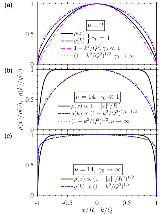
FIG. 2 (color online). Examples of the initial density profile \rho(x) (black solid lines) and the quasimomentum distribution g(k) (blue dash-dotted lines), which determines the shape of the asymptotic density profile \rho_\infty(x, t) and the momentum distribution n_\infty(k, t) , Eqs. (5) and (7), with Q being the maximum (quasi) momentum. (a) Expansion from a harmonic trap, with the solid and dash-dotted lines corresponding to the numerical results for \gamma_0 = 1 . The analytic results (coinciding with the hydrodynamic self-similar solutions) in the weakly ( \gamma_0 \ll 1 ) and strongly ( \gamma_0 \rightarrow \infty ) interacting regimes are shown, respectively, by the dashed-magenta and dotted-red lines. The numerical results in these regimes, obtained for \gamma_0 = 2.5 \times 10^{-4} and \gamma_0 = 200 , are indistinguishable from the respective analytic curves and are omitted from the graphs for clarity. (b) Main curves are for a highly anharmonic trap with \nu = 14 [27] and \gamma_0 \ll 1 ; the semicircle (dashed red line) corresponds to the limiting behavior of g(k) for a box potential ( \nu \rightarrow \infty ). (c) Strongly interacting regime, for the same \nu = 14 .
