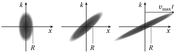
FIG. 1. Illustration of the evolving local quasimomentum distribution f(k, x; t) = f(k, x - \hbar kt/m; 0) , where v_{\max} = \hbar k_{\max}/m .
